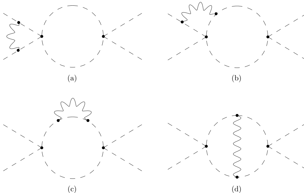
Figure 1: Representative graphs that contribute at order g^2\lambda^2/(16\pi^2)^2 . Summing all such diagrams yields an SU(4) symmetric quartic.
